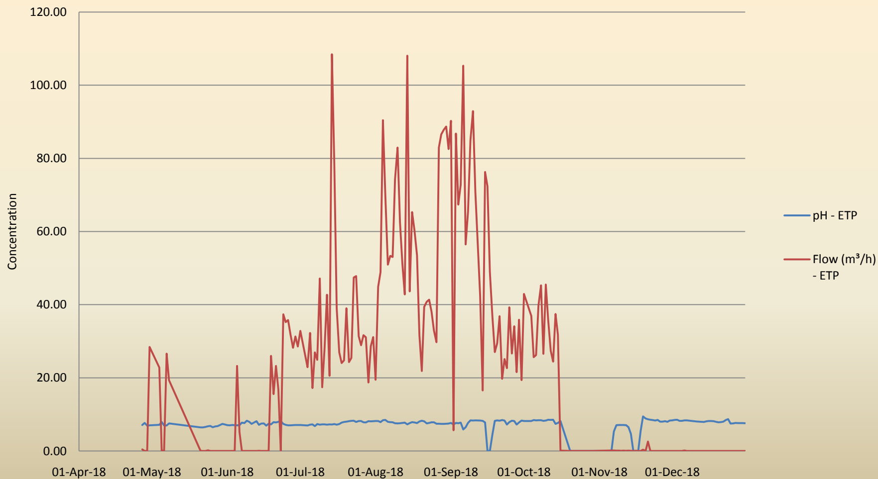
Annual Effluent Trend in M/s. Hindalco Industries Ltd., Dist. Singrauli (M.P.)
